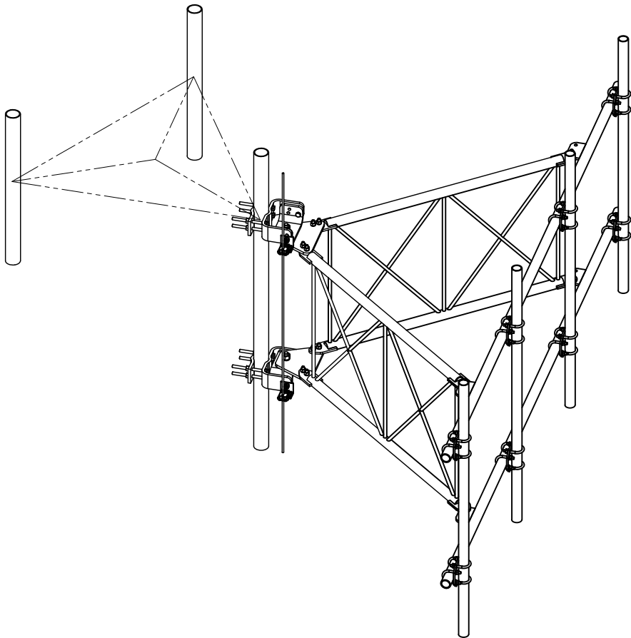
ISOMETRIC VIEW
