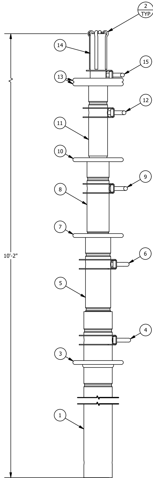
COLLAPSED VIEW
