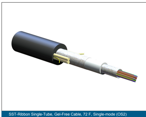
SST-Ribbon Single-Tube, Gel-Free Cable, 72 F, Single-mode (OS2)
