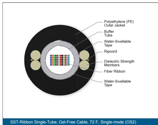
SST-Ribbon Single-Tube, Gel-Free Cable, 72 F, Single-mode (OS2)
